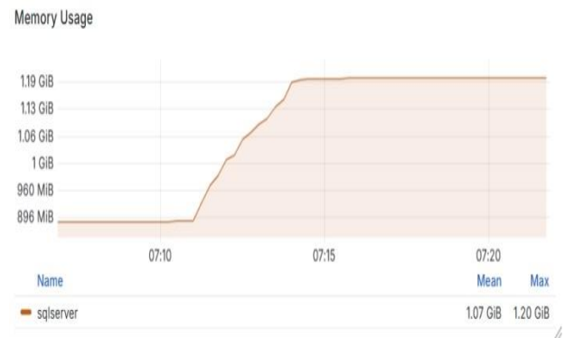
Figure 11 5K inserts memory usage SQL server
